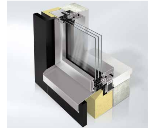
FWS 60 CV Lochfenster
